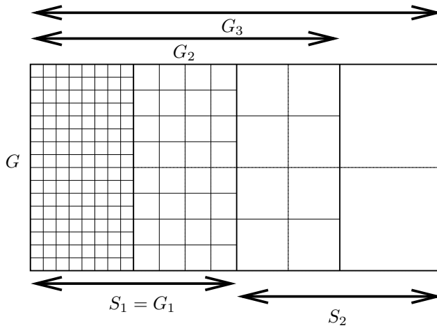
Figure 1. Subdomains G_k and S_k .
