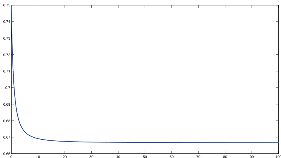
Figure 2: Condition (3.12) for p(t) = \frac{t^3}{1+t}
