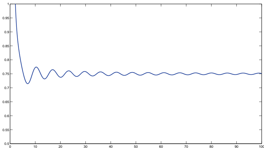
Figure 1: Condition (3.12) for p(t) = t^3 + t \cos(t)
