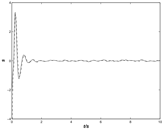
Fig. 2. Sliding surfaces.
