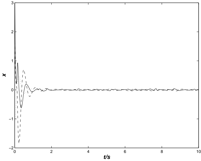
Fig. 1. State response.
