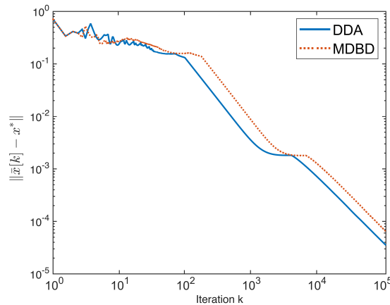
Fig. 2: The comparison between our DDA algorithm and the MDBD algorithm.
