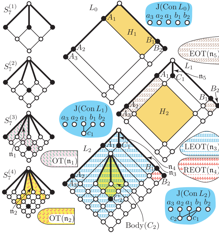
Figure 2. Multifork extensions and some geometric objects.
