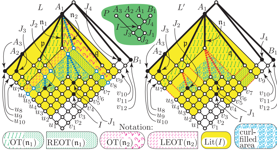
Figure 4. Illustrating the proof of Lemma 4.6 by \text{Lamp}(L) \cong P \cong \text{Lamp}(L') .
