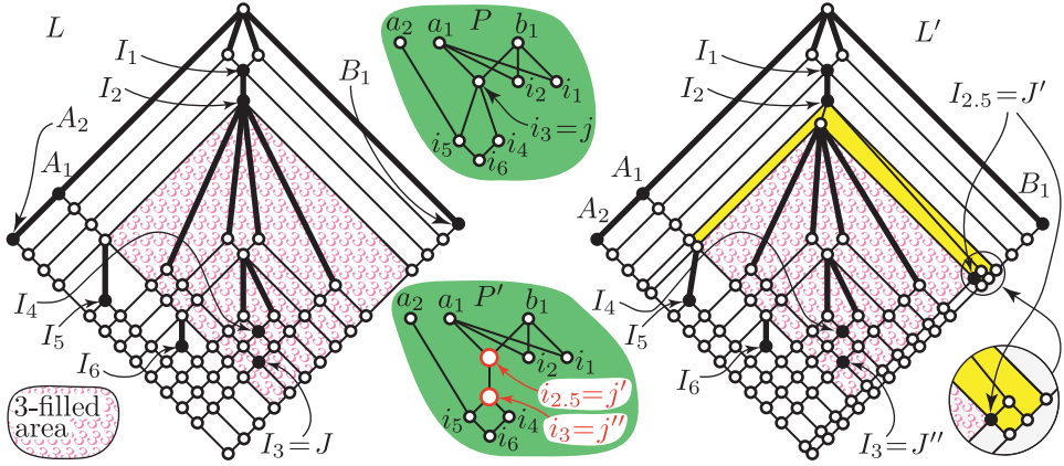
Figure 5. The construction for Proposition 6.1 with a “magnifying glass” at the bottom right.
