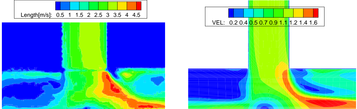
Figure 14: Velocity in the channel junction – experiment (left) and simulation (right).
