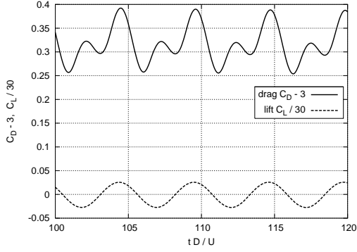
Figure 1: Laminar flow around cylinder, \beta = U .
