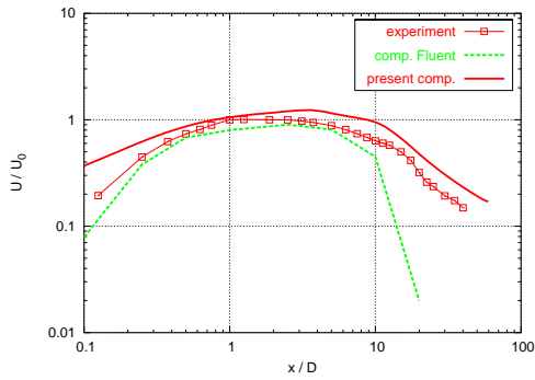
Figure 10: Time averaged velocity on the jet axis.
