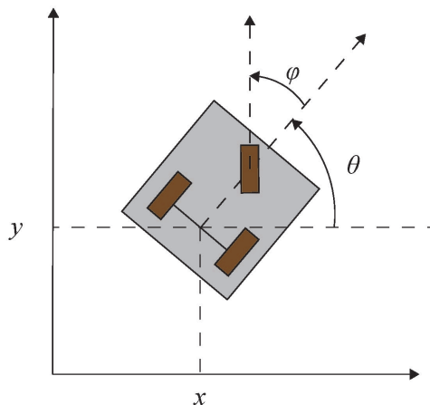
Fig. 3. A front wheel car model.
