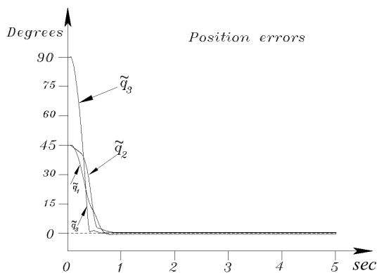
Fig. 7. Position errors of the hyperbolic controller, case m=3 .
