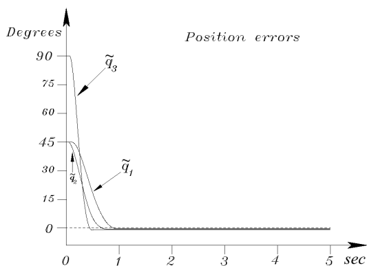
Fig. 9. Position errors of the PD control.
