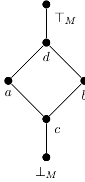
Fig. 1. Hasse diagram of M .
