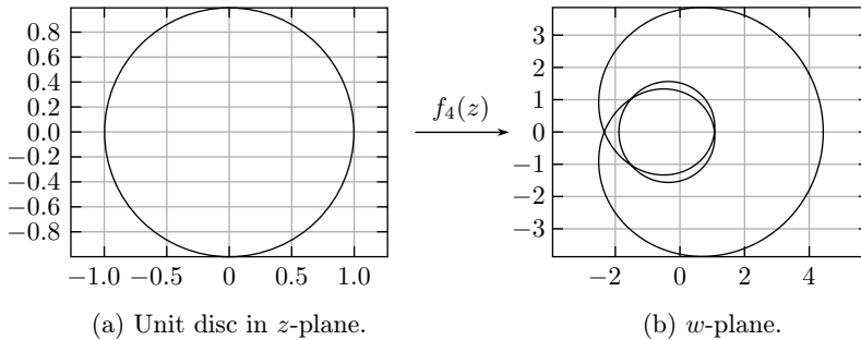
Figure 3. Pictorial representation of f_4(z) = z + 1.2725z^2 + 2.1701z^3 + \dots
