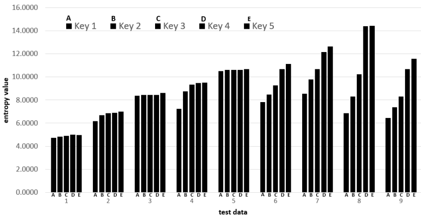
Fig. 8: Average entropy values for each MMPLS-IWevelet type for each ciphertext test data for several key variances.
