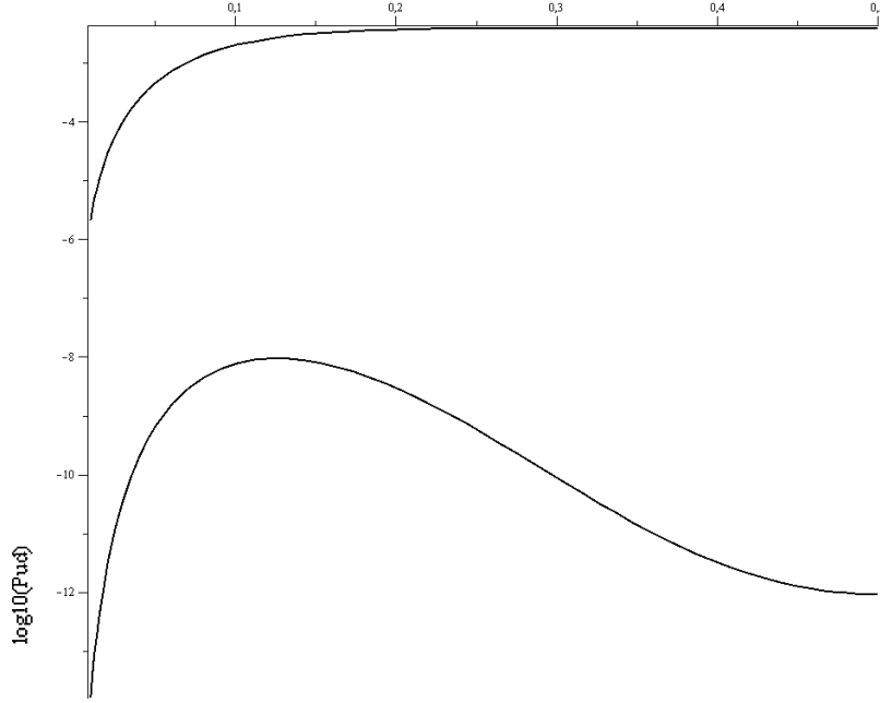
Figure 1: The probability of an undetected error for the sample code (upper curve) and for the same code combined with repetition of the message. Horizontal axis: bit error rate p_e , vertical axis: logarithm of probability of undetected error P_{ud}(p_e) .
